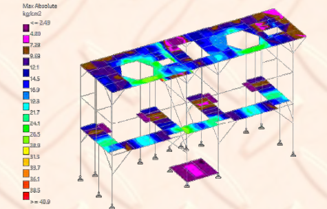
Stainless checked plate 4 mm. stress, maximum = 40.9 kg/cm2 < 0.6fy = 0.6x2,400 = 1,440 kg/cm2 (Pass)
