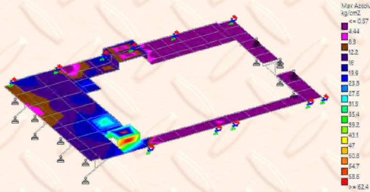
Checked plate 4.5 mm. stress, maximum = 62.4 kg/cm2 < 0.6fy = 0.6x2,400 = 1,440 kg/cm2 (Pass)
