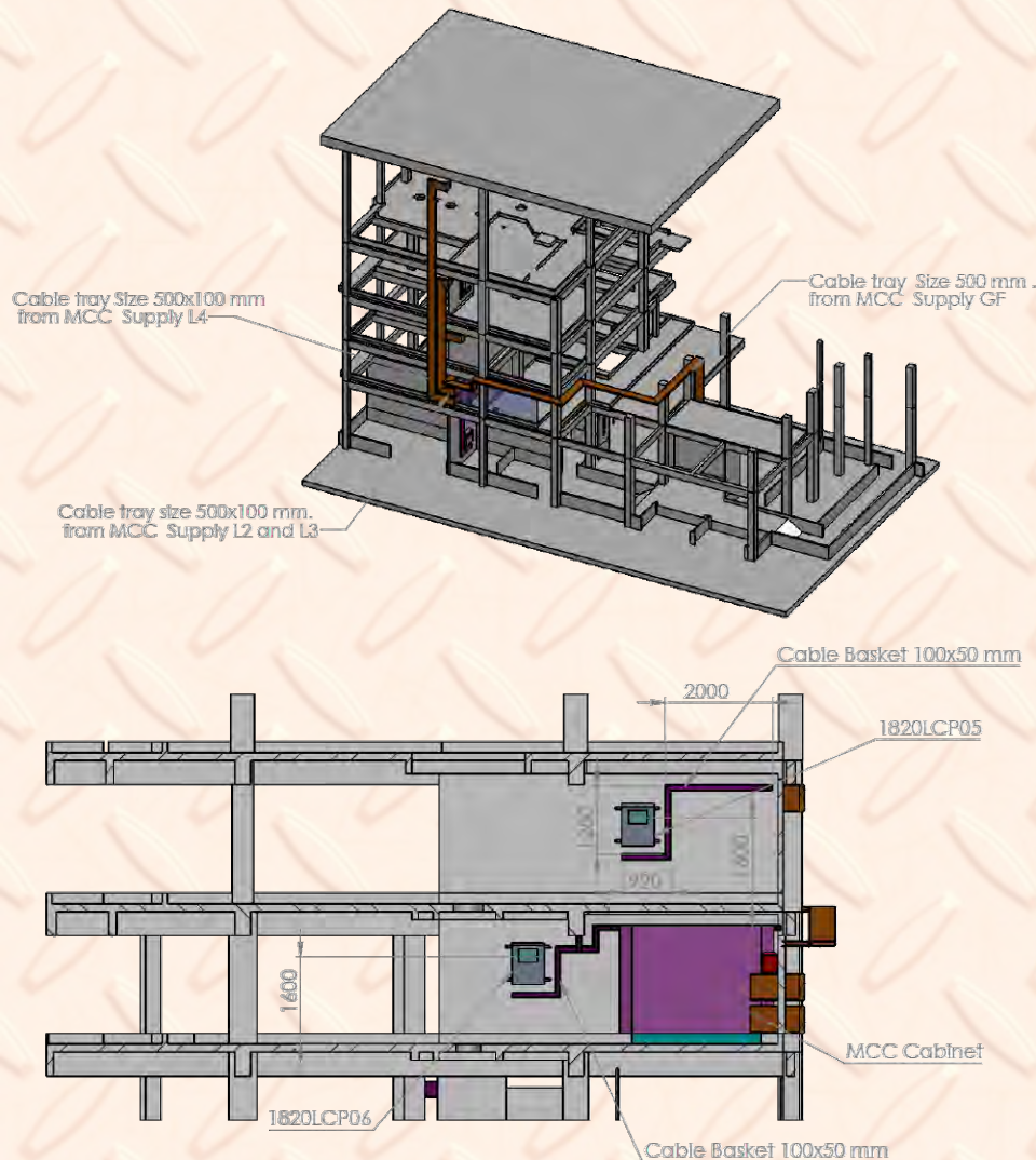
3D Cable Routing Layout Drawing
