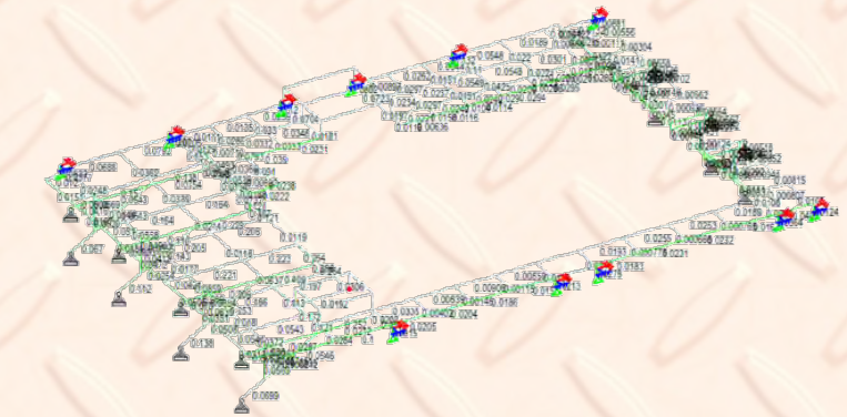
Steel design ratio of steel platform (Overall < 1.00 Pass)
